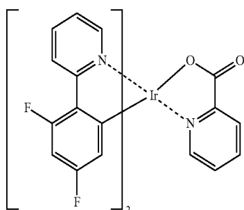
F 2 Irpic
